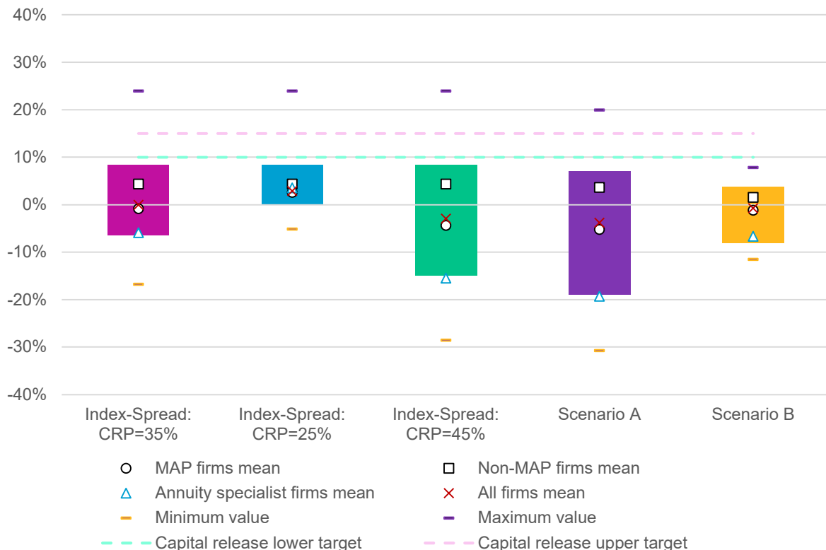
Figure 4.1: Percentage change in OF after allowing for TMTP recalculation
