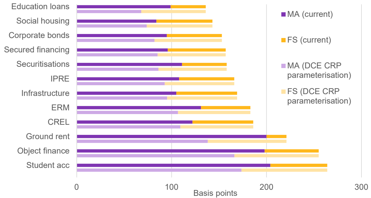
Figure 3.7: Comparison of MA and FS in basis points (based on current FS and CRP parameterisation adopted within the DCE) for different asset classes at year-end 2020
